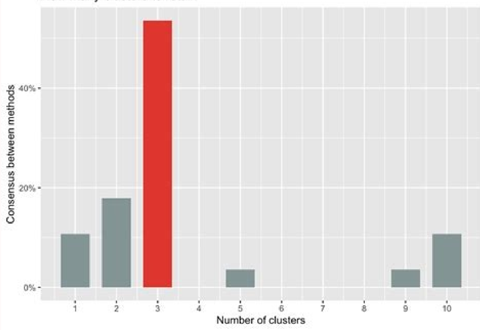
How many clusters to retain
